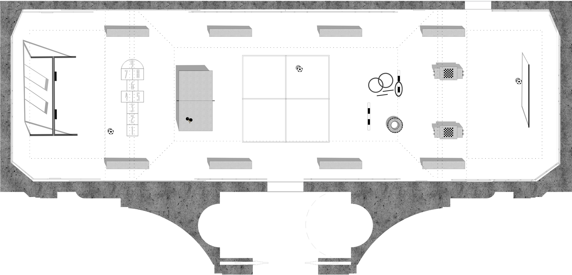
PLAN | PLAN 1:100
