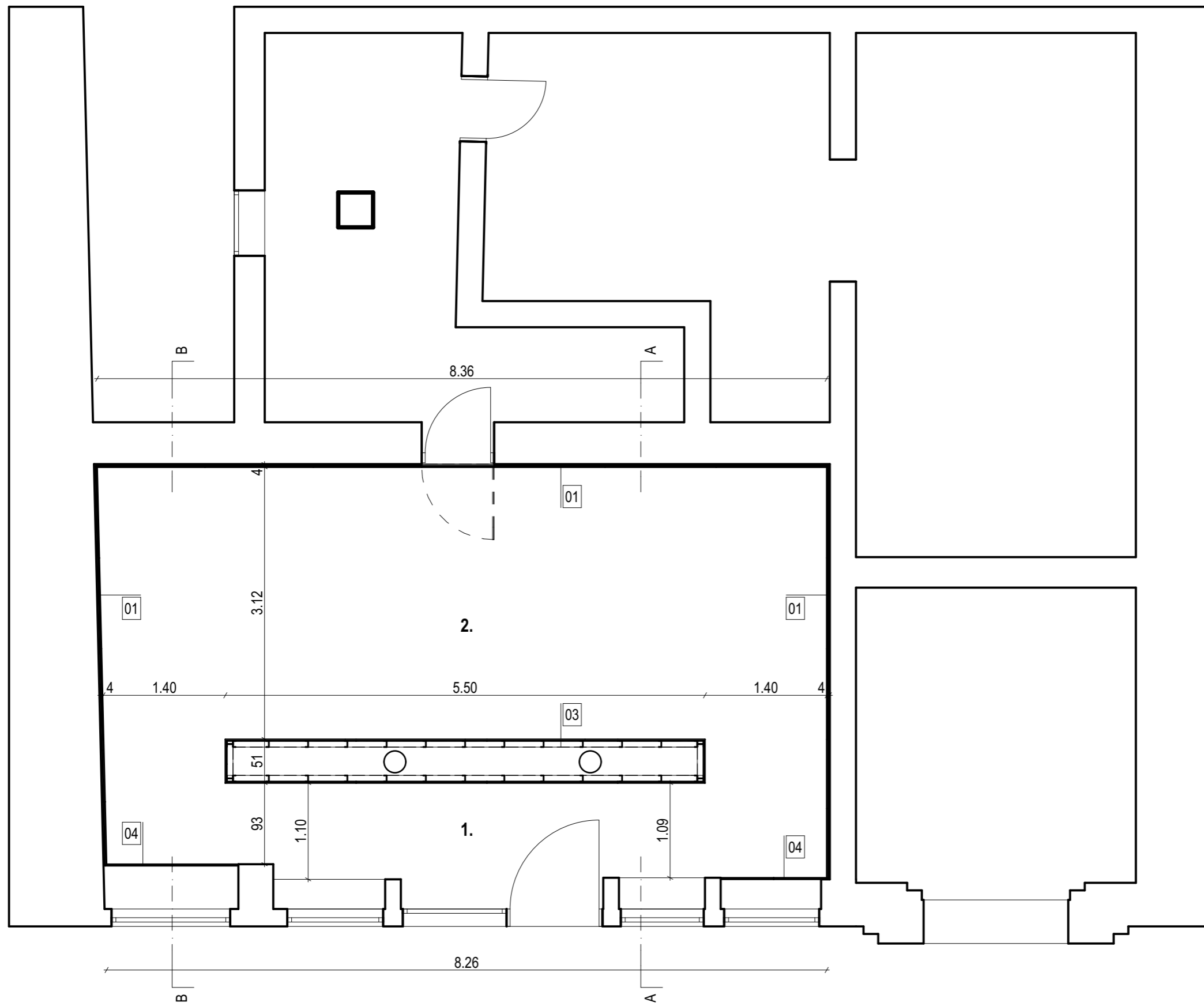
PLAN/FLOOR PLAN
